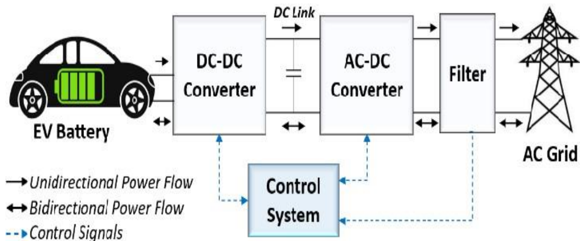
Fig. 1. Block diagram of Fast Charging EV Station
