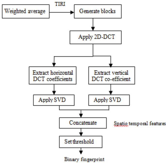
Fig 1: Fingerprint Generation
